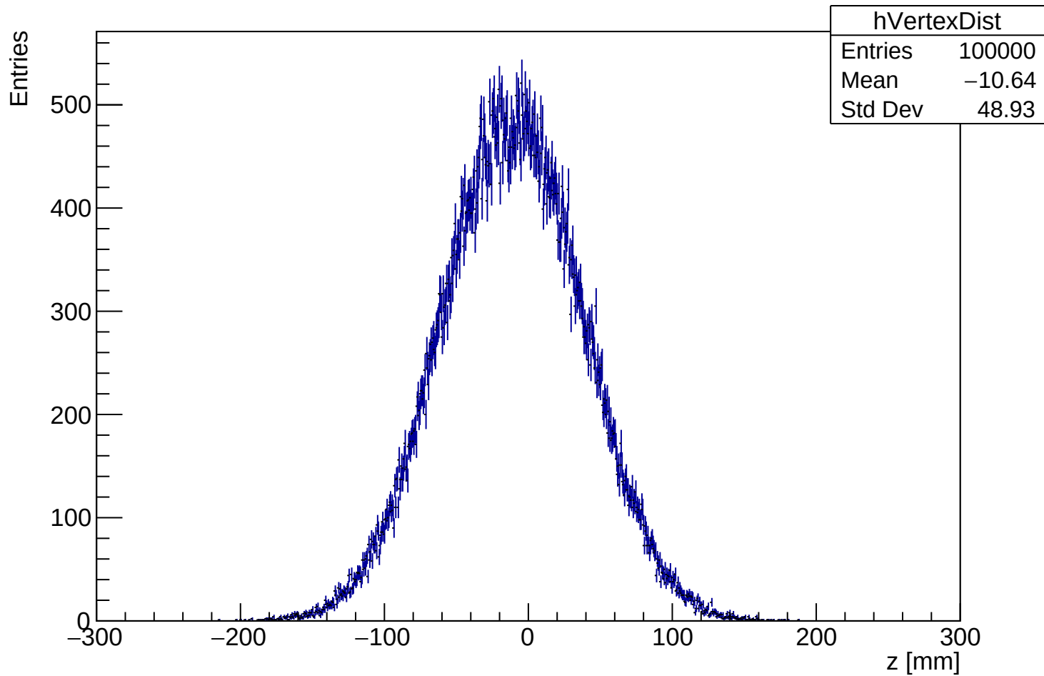
Distribution of the interaction vertex along the z-axis
